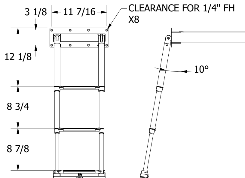
DEPLOYED VIEW SCALE 1 : 12
