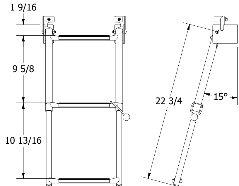
DEPLOYED VIEW SCALE 1 : 8
