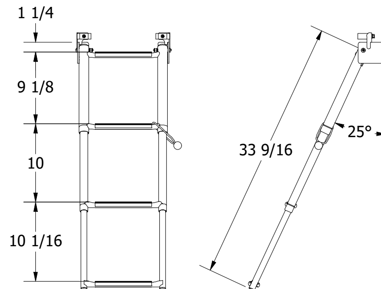
DEPLOYED VIEW SCALE 1 : 12
