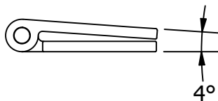
FOLDED VIEW
