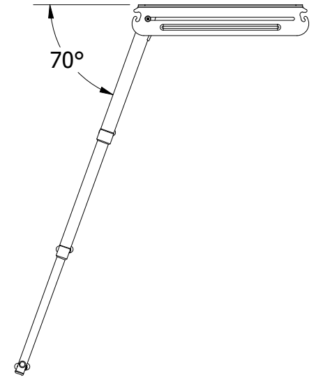
DEPLOYED VIEW SCALE 1 : 12
