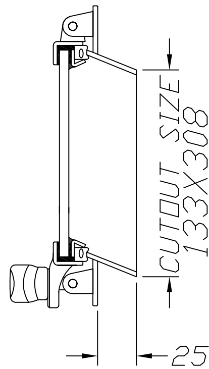
ANGLED TYPE
